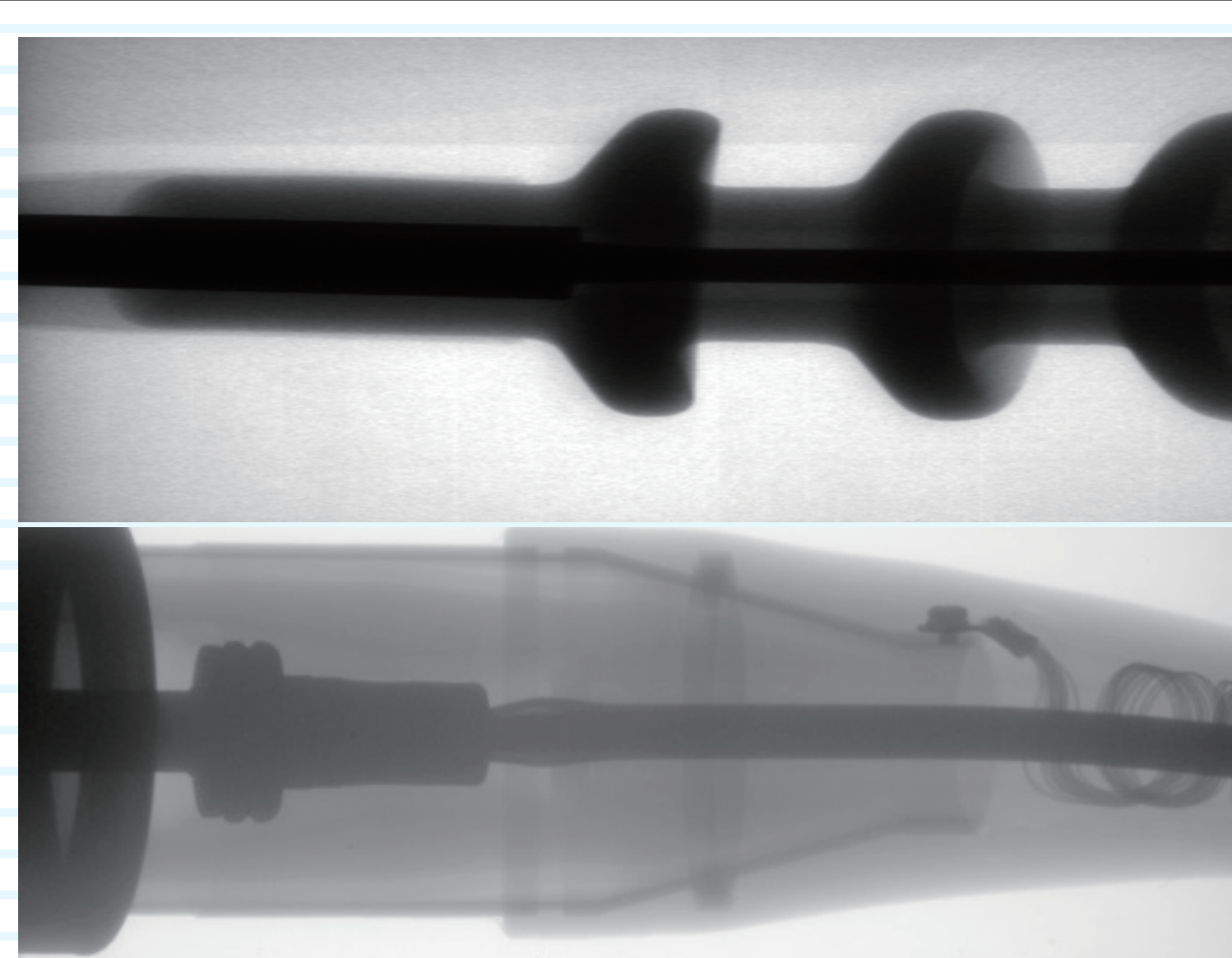
Wire end inspection
