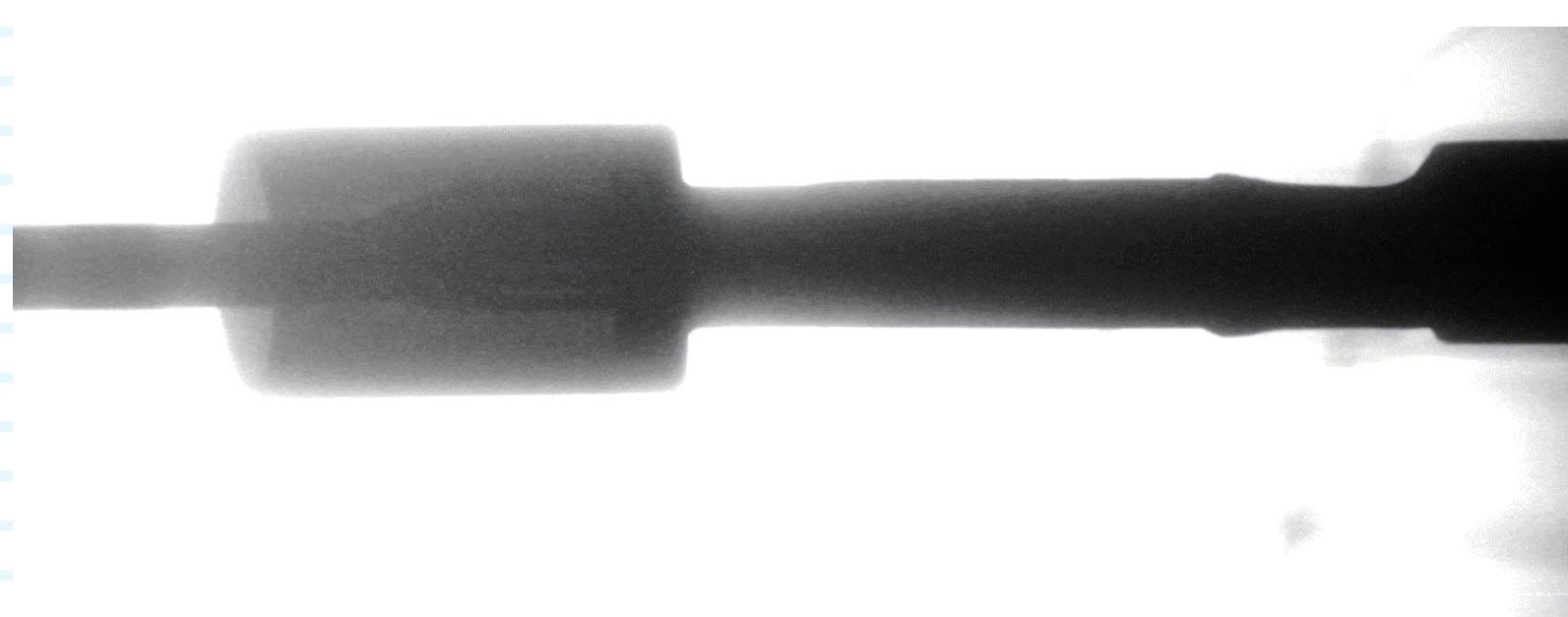
Image of X-ray inspection for a wire sample
